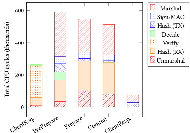
Figure 6: The aggregate cost of each pipeline stage in a domain-optimized setup (in CPU cycles) at the leader for 15 nodes, processing 4KB values, shows that (un)marshaling and hashing before verification are the most expensive.
