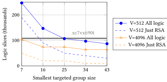
Figure 11: Estimated resource consumption of a 10Gbps PBFT implementation on FPGAs using open-source components targeting a minimum value size and group size.
