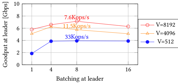
Figure 9: ModuBFT takes advantage of the 10Gbps bandwidth available at the leader, but to achieve an almost complete utilization of it some amount of batching is necessary.
