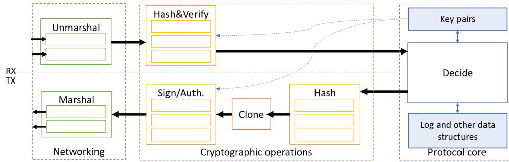
Figure 4: In ModuBFT, the consensus logic is implemented as a software pipeline, with data parallel execution for compute-intensive steps.
