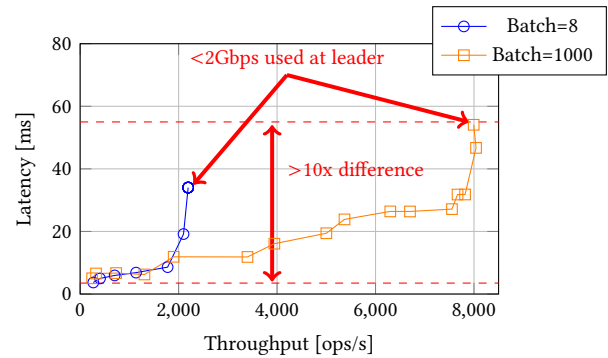
Figure 1: State-of-the-art BFT consensus libraries fail to efficiently utilize 10Gbps LAN connections (BFT-Smart with 7 nodes, 4KB payload, no logging)
