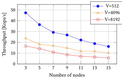
Figure 7: Increasing the number of nodes has a predictable impact on throughput. The leader node becomes bound on its network stack for larger group sizes.
