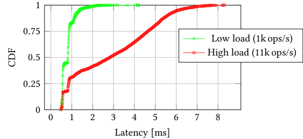
Figure 10: ModuBFT implementation highlights additional opportunities for HW: reducing the long tail of response times under load (15 nodes and 4KB payload)
