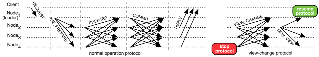
Figure 3: PBFT communication pattern during failure-free operations and recovery.
