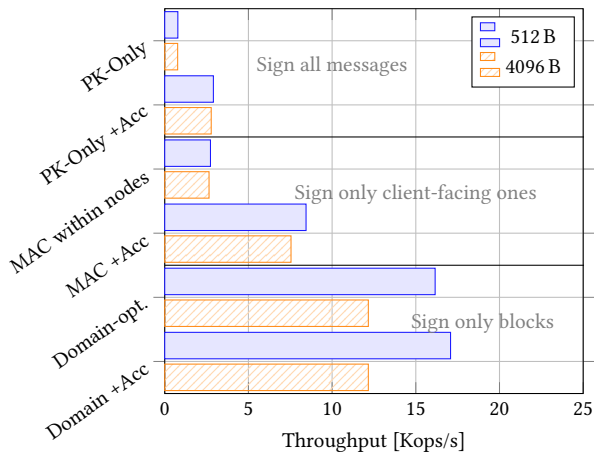
Figure 5: We emulate different configurations with 15 nodes to quantify the expected benefits of hardware accelerators and protocol optimizations. The results show that the avoidance of PK cryptography is the most important performance factor.
