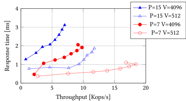
Figure 8: Even under load ModuBFT delivers response times that increase predictably. For small values it is possible to keep response times under 2ms even when fully saturated.
